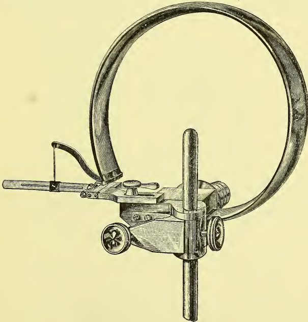
FIG. 42. FICK'S SPRING MANOMETER.
